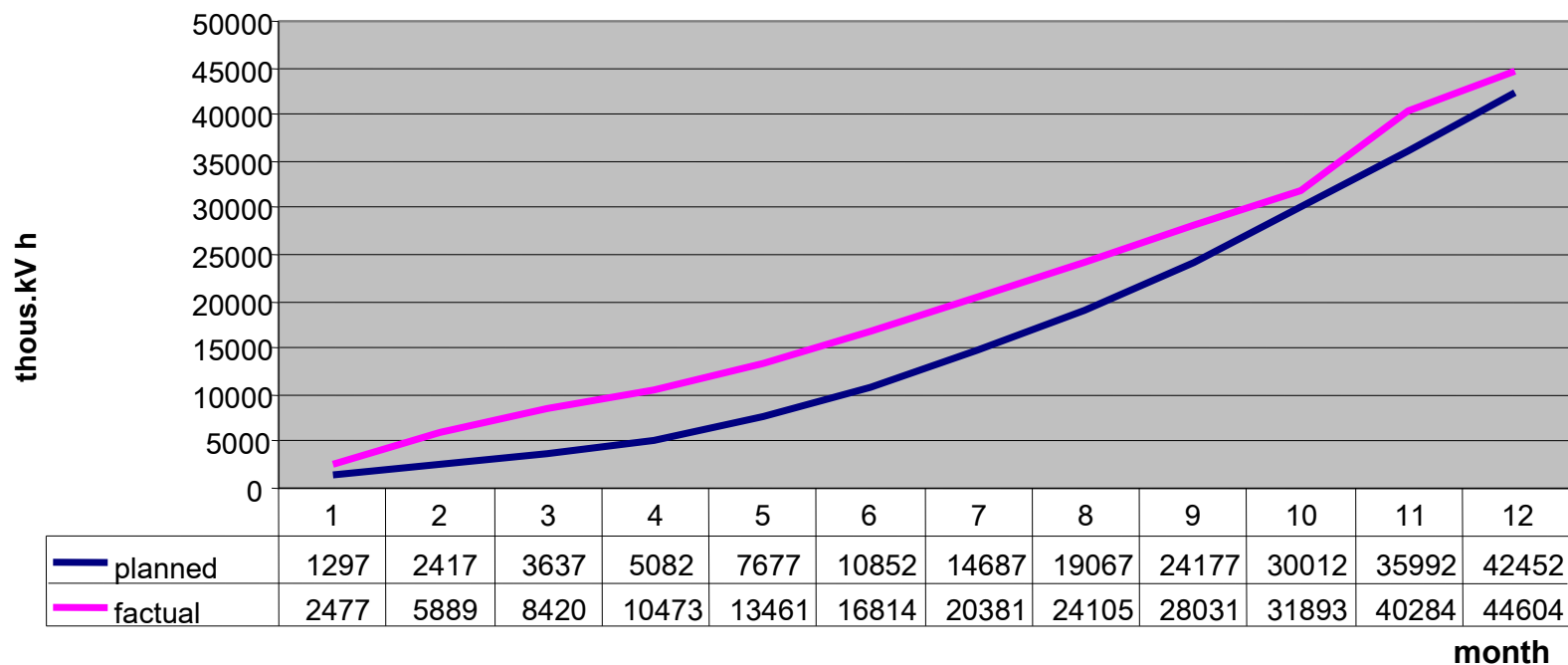
DIAGRAM Of energy savings in 0,4-110 kV el. networks of "ENA" CJSC for 2005
